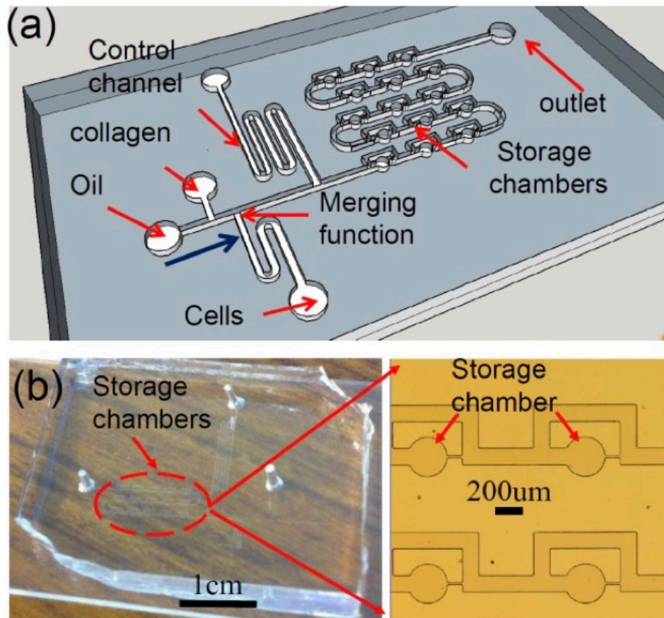
Figure 12. (a) Sketch of the droplet microfluidic device for generating 3D microtissues: Each storage chamber (a cylinder with a radius of 180\ \mu\text{m} and height of 30 or 80\ \mu\text{m} ) has one 3D microtissue containing single or multiple cells; (b) photo of a fabricated chip with 15 storage chambers; (c) optical micrography showing the storage chambers
